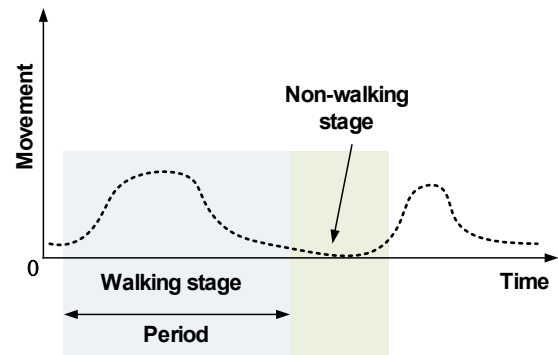
Figure 2 –Spatio-temporal movement
